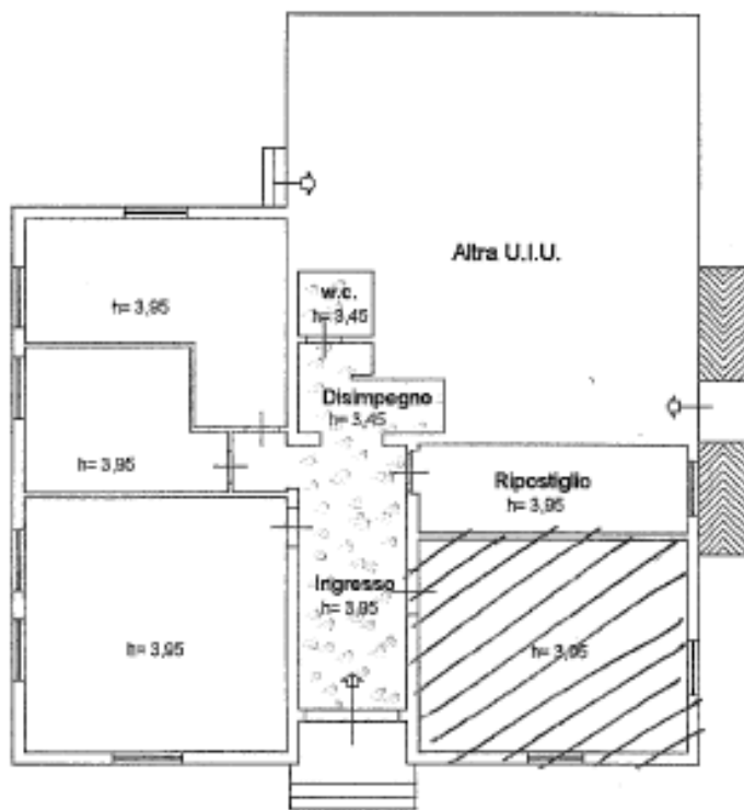
PIANO TERRA
